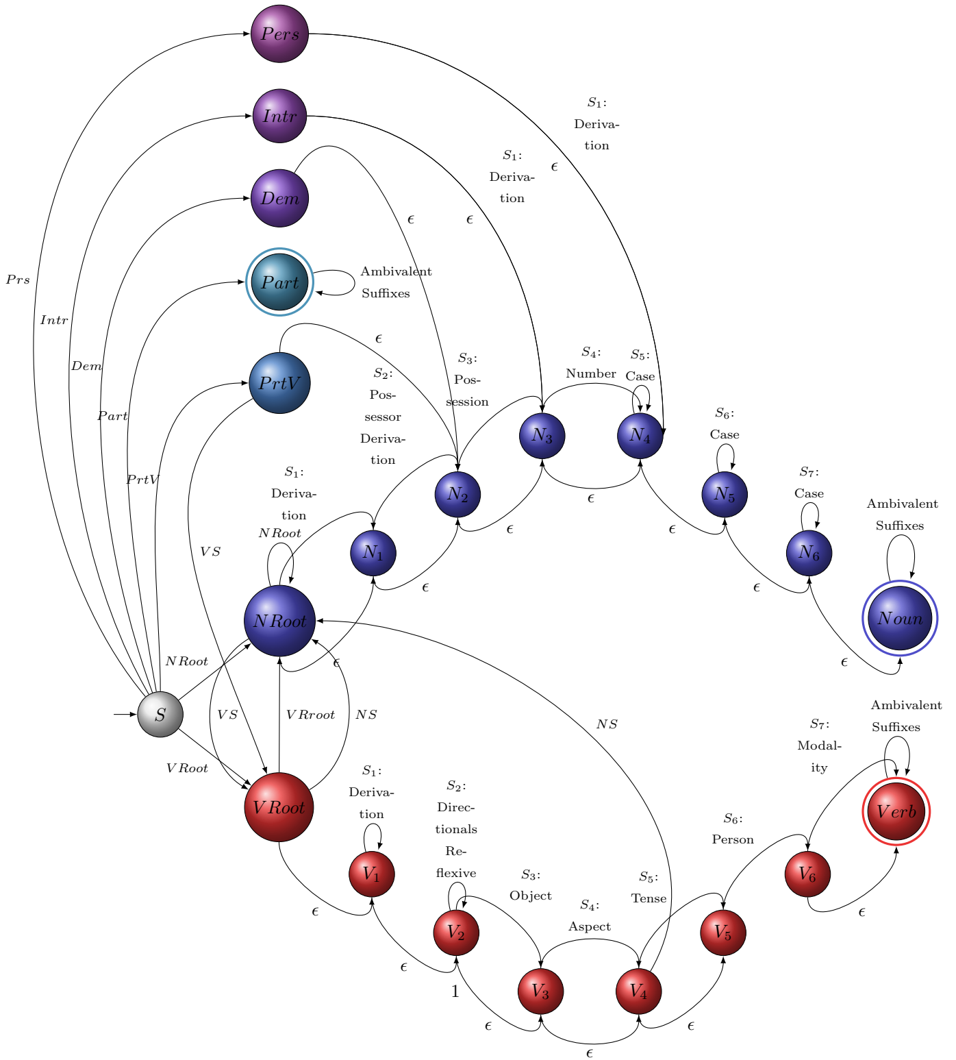
Figure 1: Simplified Quechua Suffixes Transducer
